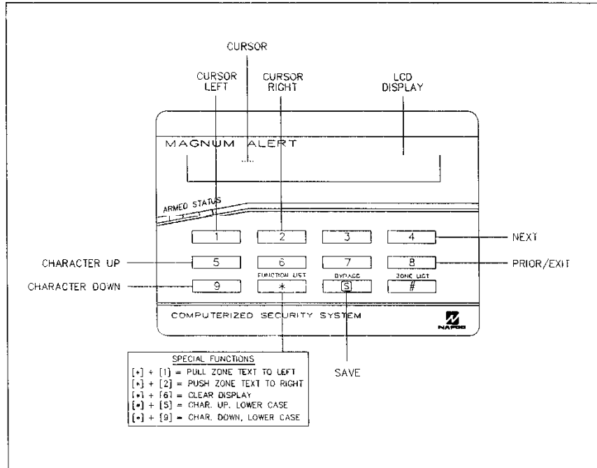
Keypad functions, Program Mode.
